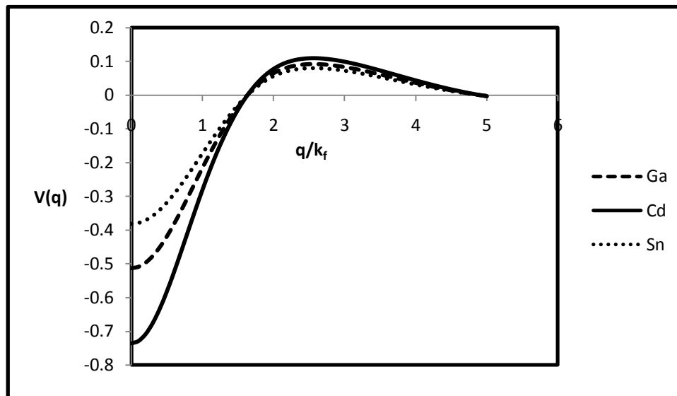
Fig. 1. Form factors of Ga, Cd and Sn.
